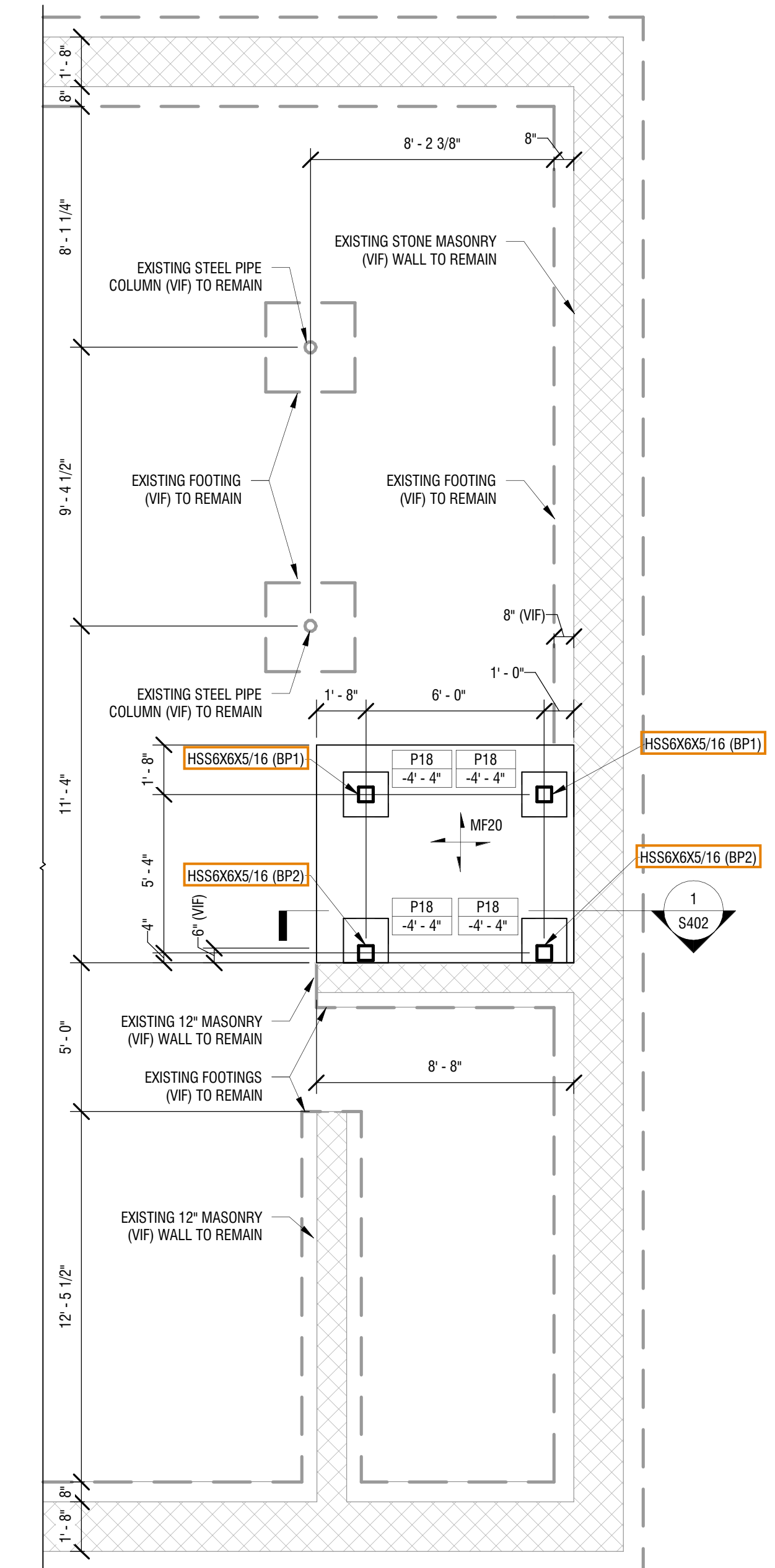
1 S401 1/4" = 1'-0"
