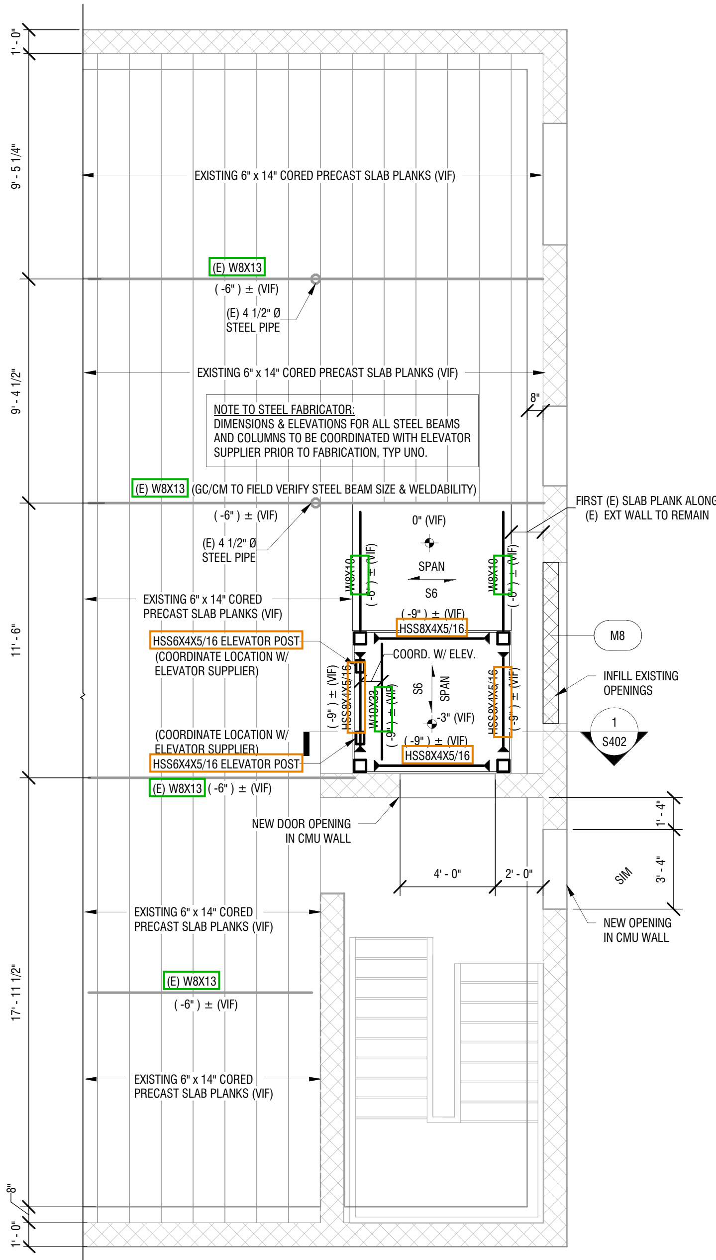
2 S401 1/4" = 1'-0"
